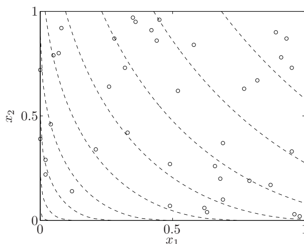
Figure 6.25 Forty goods baskets a_1, \dots, a_{40} , shown as circles. The 0.1, 0.2, ..., 0.9 level curves of the true utility function u are shown as dashed lines. This utility function is used to find the consumer preference data \mathcal{P} among the 40 baskets.
